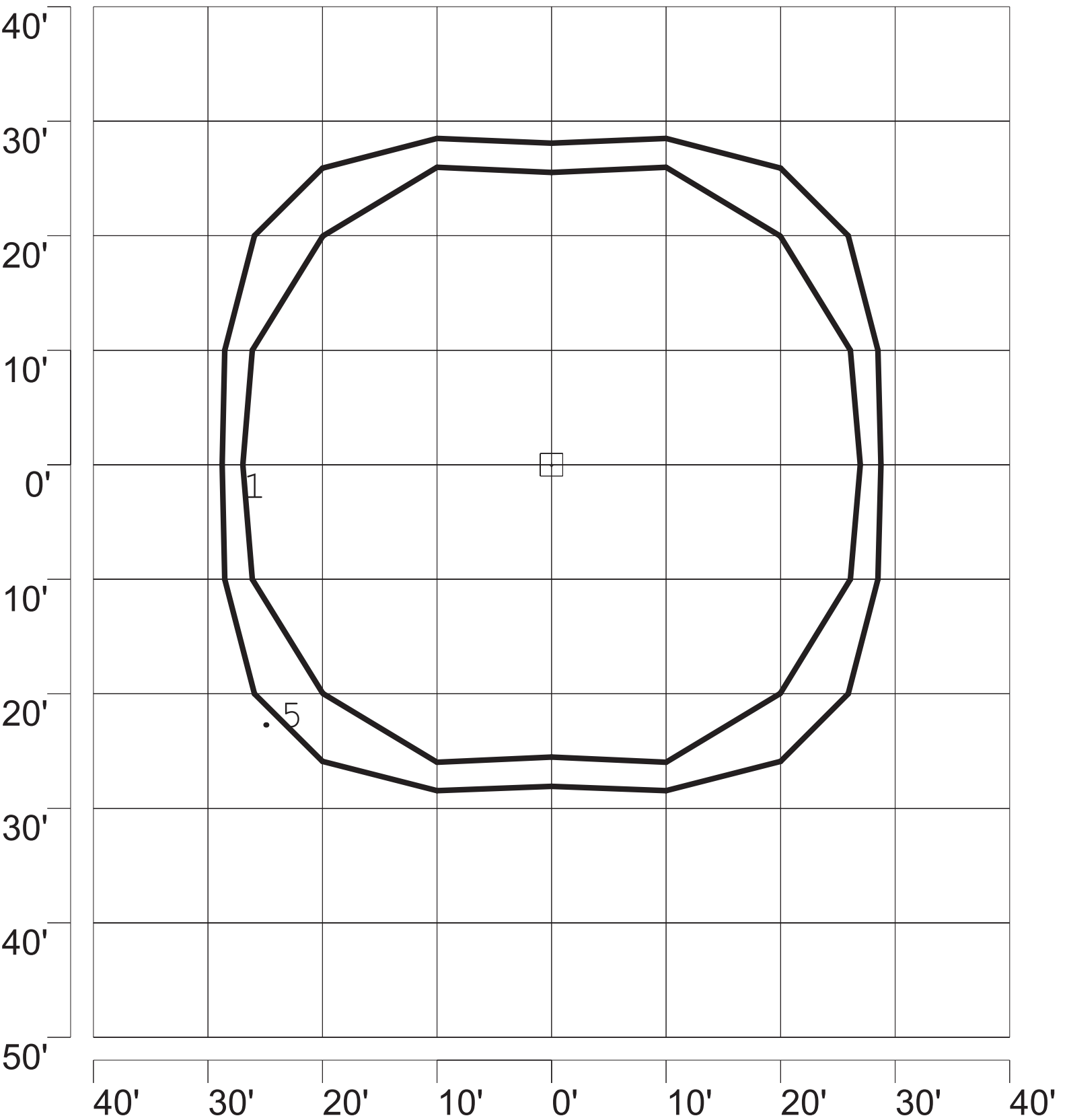
ISOFOOTCANDLE PLOT: CLG3A1 100W MH CANOPY 10' AFG - 0 DEGREE TILT
