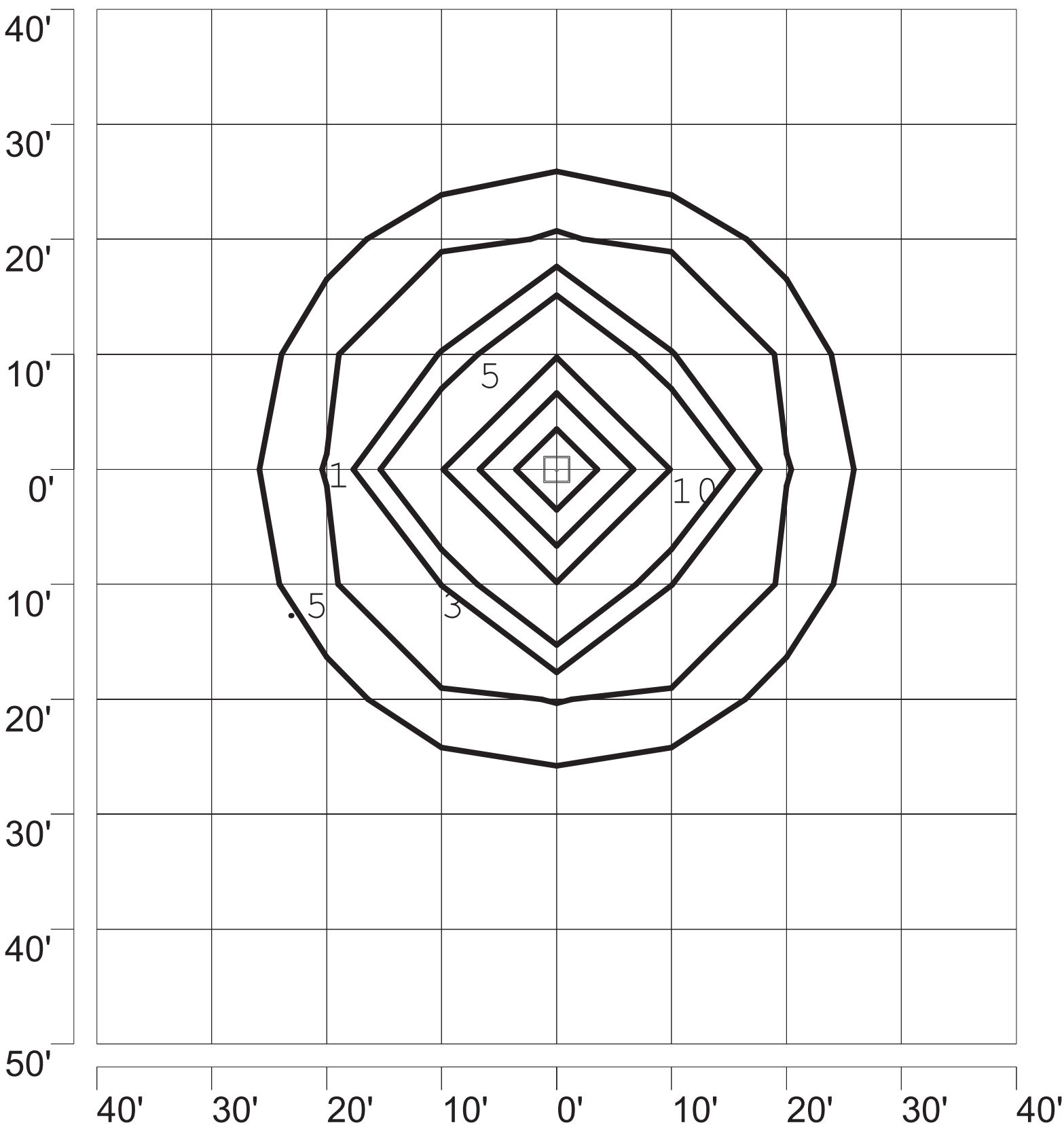
ISOFOOTCANDLE PLOT: CES-150-MT-FP 150W PSMH CANOPY 10' AFG - 0 DEGREE TILT
