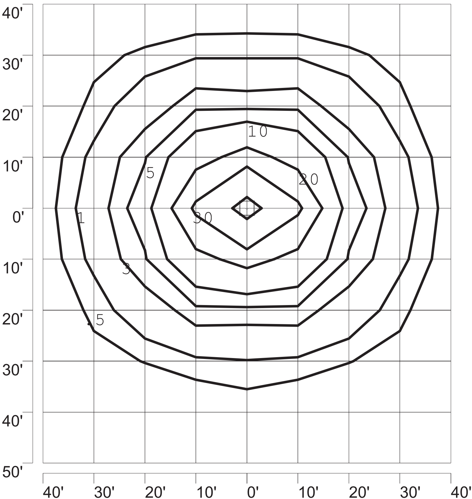
ISOFOOTCANDLE PLOT: CEM-400-MT-PS-FP 400W PSMH CANOPY 15' AFG - 0 DEGREE TILT
