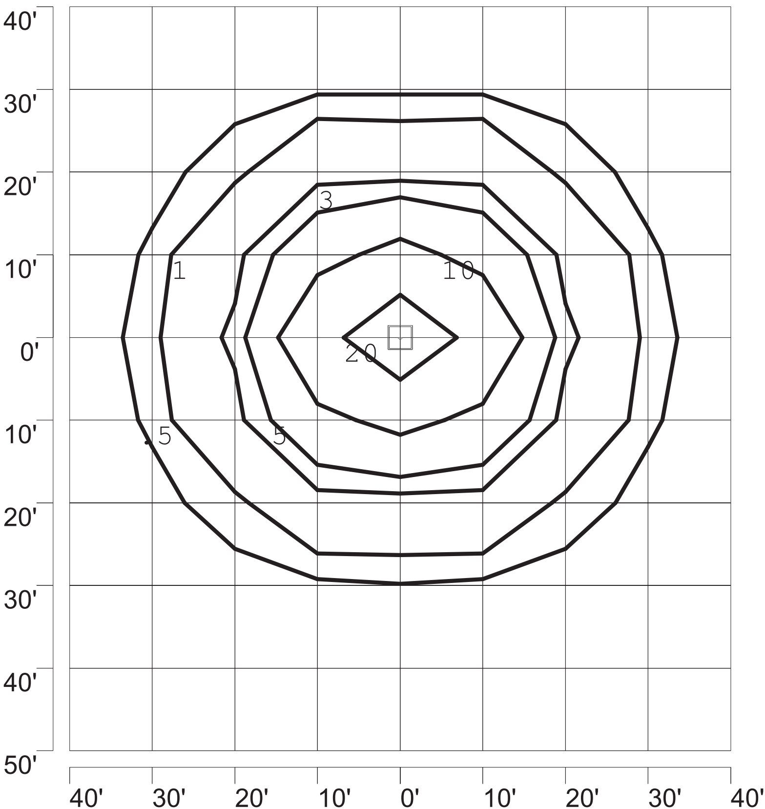
ISOFOOTCANDLE PLOT: CEM-250-MT-PS-FP 250W PSMH CANOPY 15' AFG - 0 DEGREE TILT
