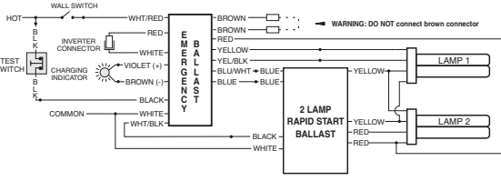
FIG R TWO (2) COMPACT LAMP RAPID START BALLAST
