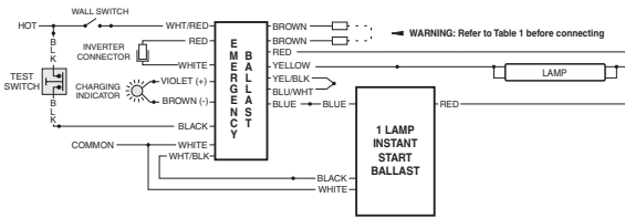
FIG B ONE (1) LAMP INSTANT START BALLAST
