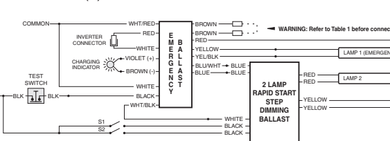
FIG K TWO (2) LAMP RAPID START STEP DIMMING BALLAST
