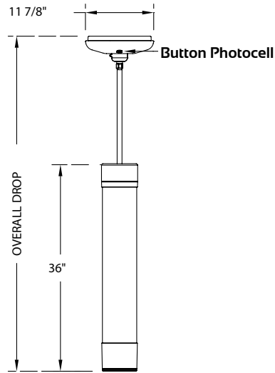
SH Stem Hung Mount
