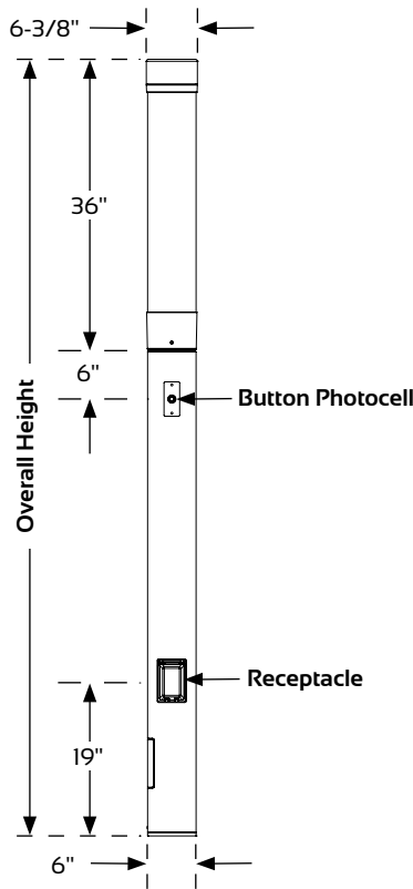
Low Profile Base For Heights ≤ 12'
