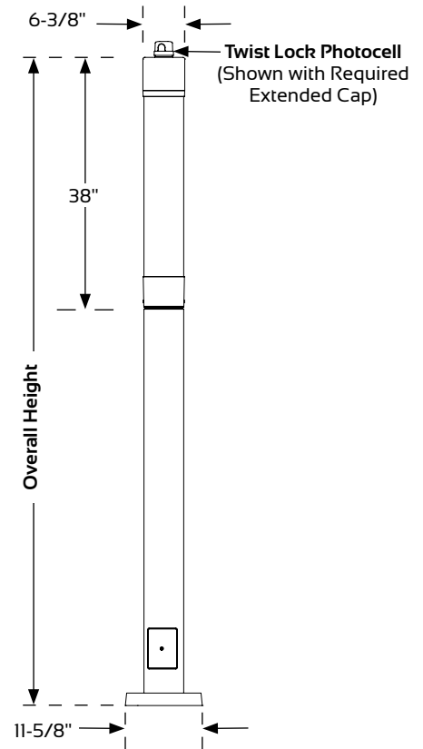
Wide Base For Heights > 12'
