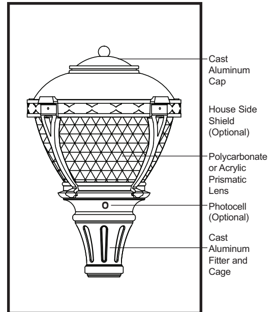
EPA = 0.79 (ft 2 ) WEIGHT = 25 LBS
