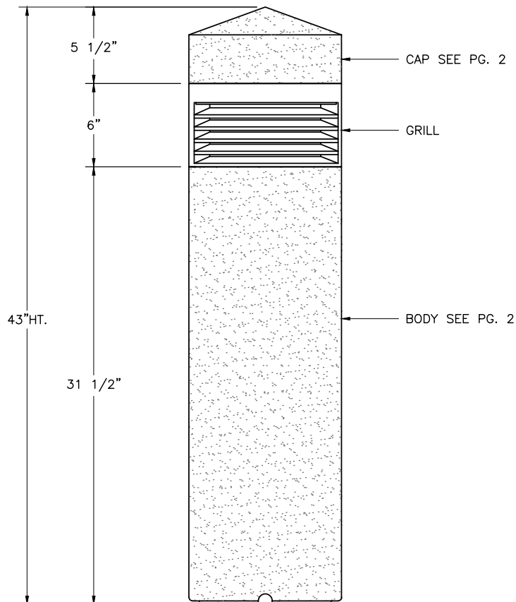
ELEVATION VIEW
