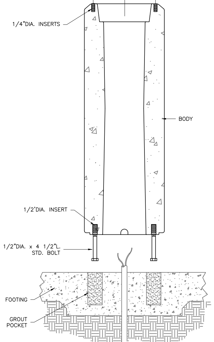
ELEVATION VIEW
