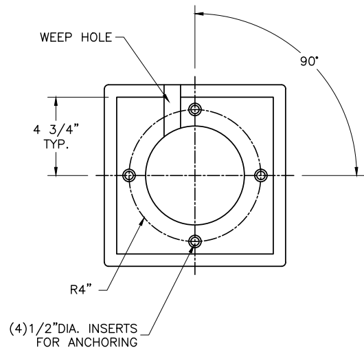
BOLLARD BOTTOM VIEW ANCHOR BOLT PATTERN
