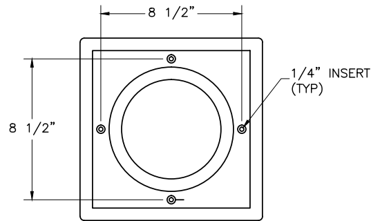
BOLLARD TOP VIEW
