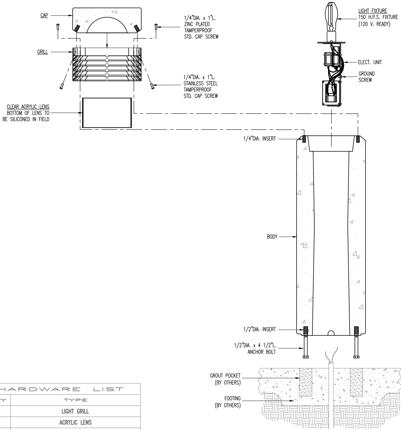
ELEVATION VIEW
