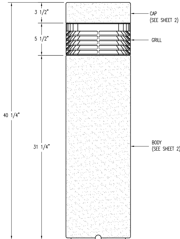
ELEVATION VIEW
