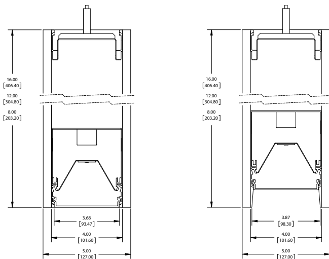
SA4xxDP Flush
