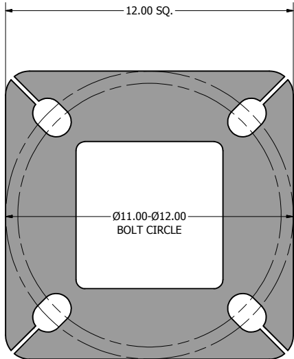
12.00 X 12.00 X 1.00 THK. BASE PLATE
