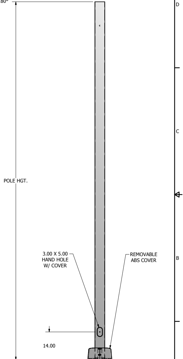
POLE DETAIL
