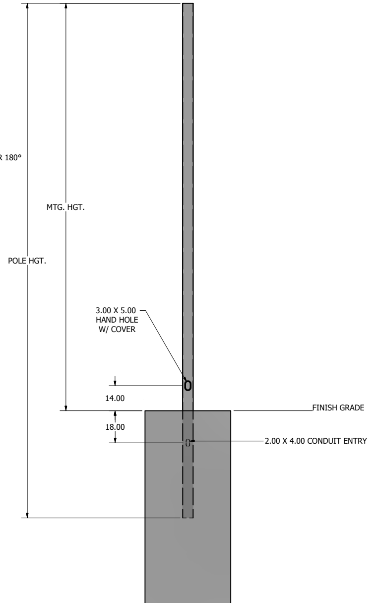
POLE DETAIL
