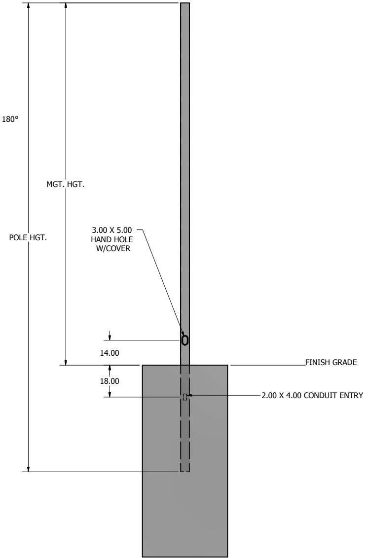
POLE DETAIL
