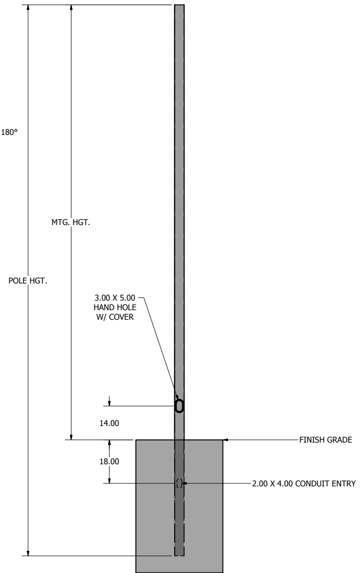
POLE DETAIL
