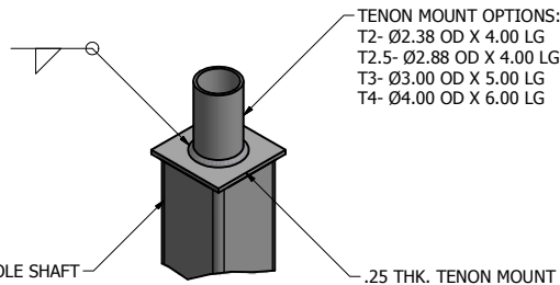
TENON MOUNT OPTIONS
