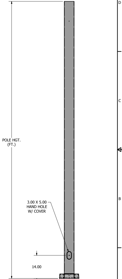
POLE DETAIL
