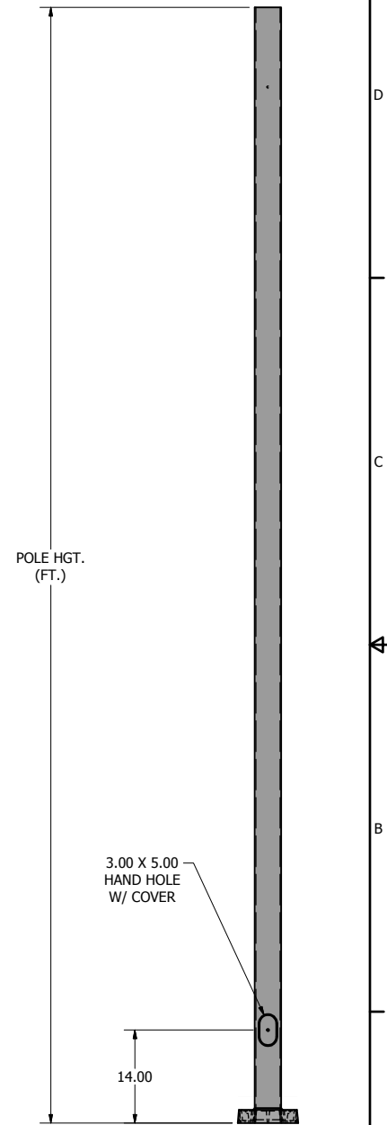
POLE DETAIL
