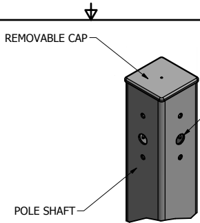
DRILLED MOUNT OPTIONS
