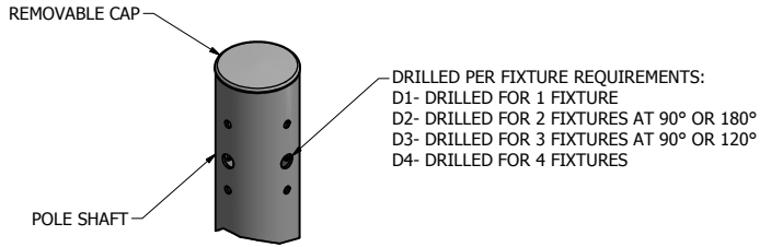
DRILLED MOUNT OPTIONS
