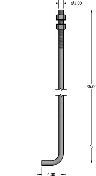
Ø1.00 X 40.00 ANCHOR BOLT
