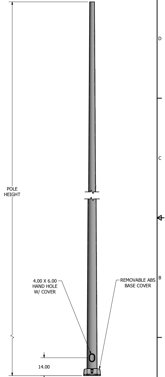
POLE DETAIL
