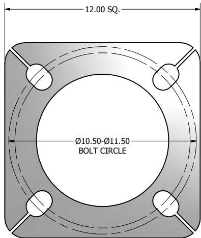
12.00 X 12.00 X 1.00 THK. BASE PLATE
