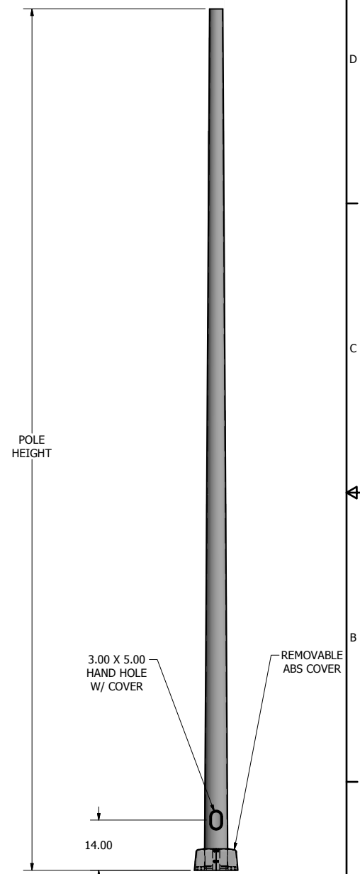
POLE DETAIL
