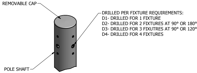
DRILL MOUNT OPTIONS
