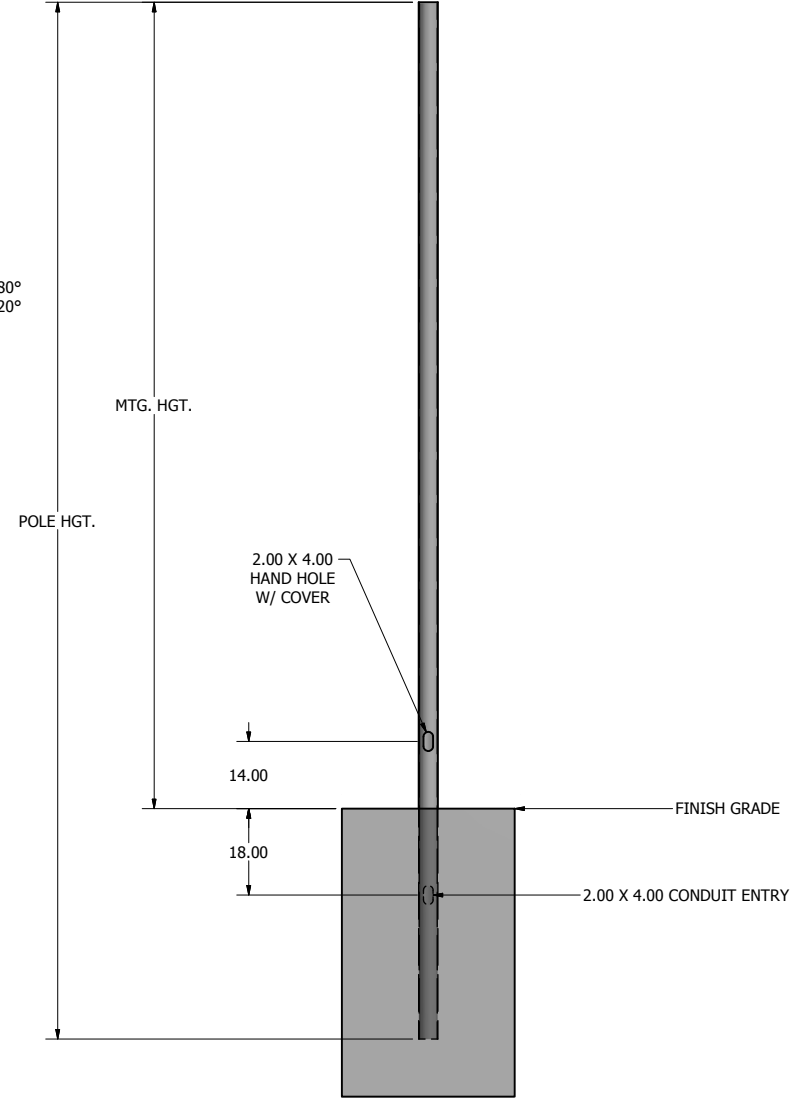
POLE DETAIL
