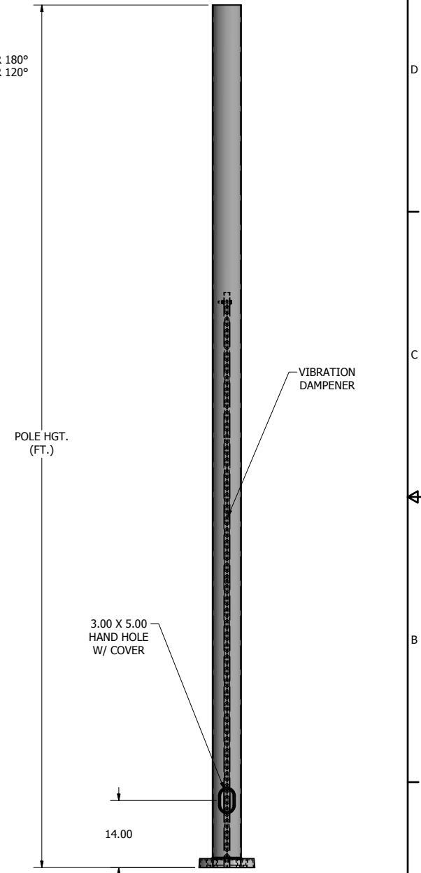
POLE DETAIL
