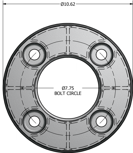
Ø10.62 X 1.88 THK. BASE CASTING
