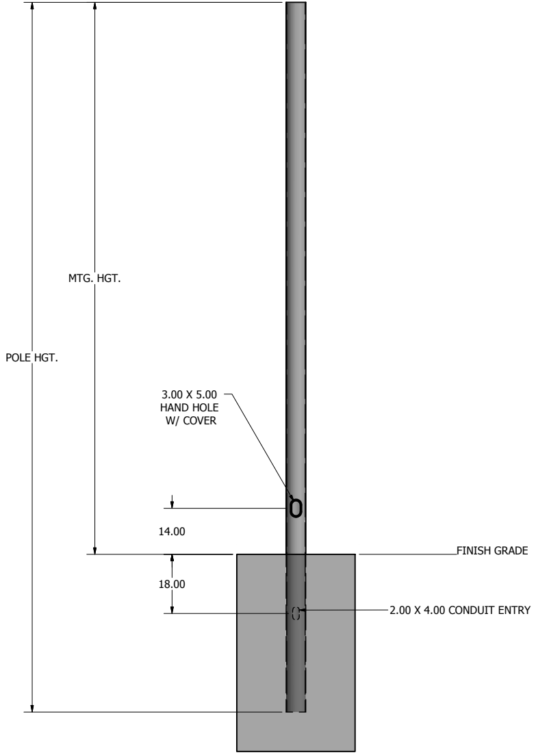
POLE DETAIL
