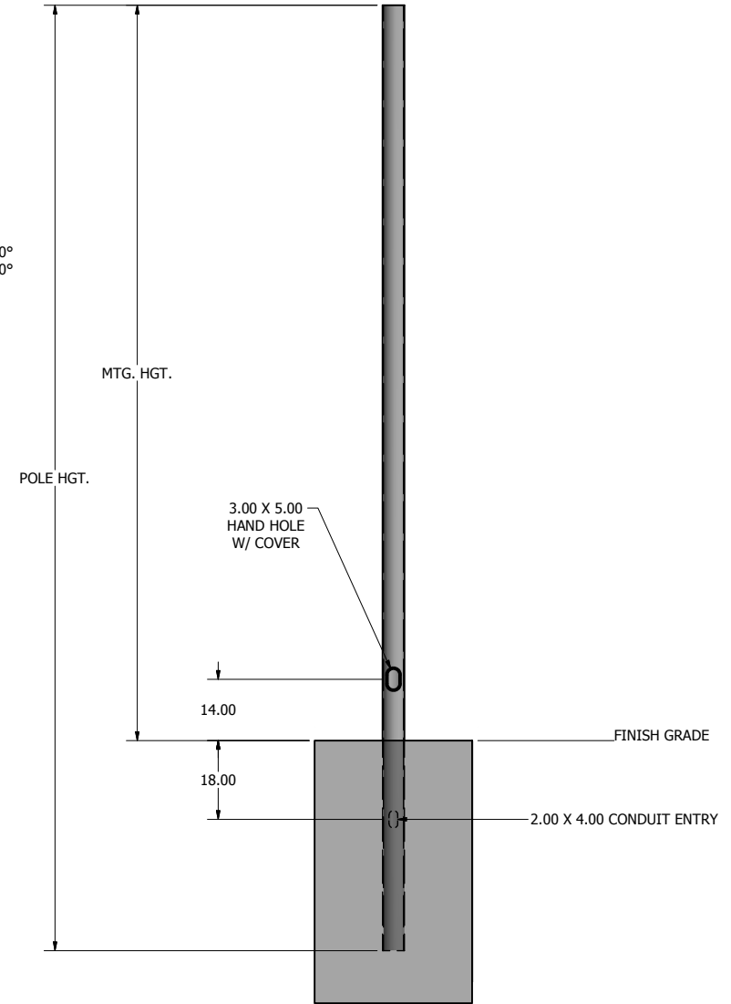
POLE DETAIL
