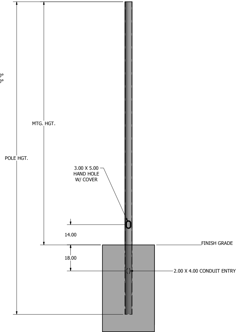
POLE DETAIL
