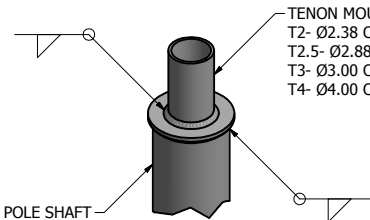
TENON MOUNT OPTIONS
