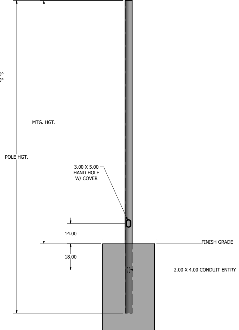
POLE DETAIL
