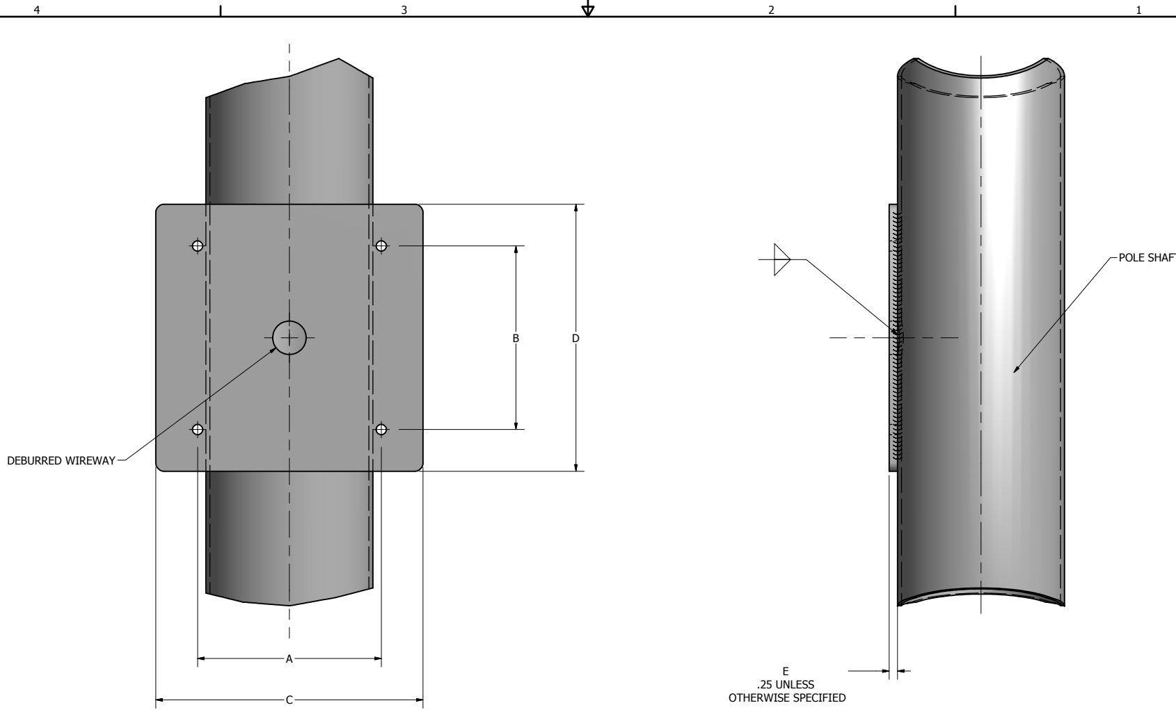
CAMERA MOUNTING PLATE DETAIL
