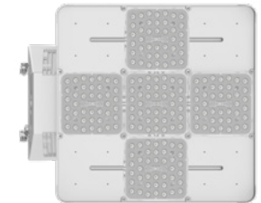
5 board configuration (Up to 77,000 lumens)
