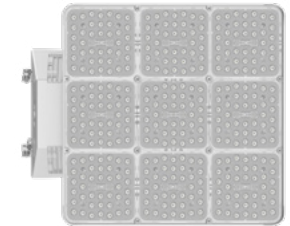
9 board configuration (Up to 132,000 lumens)
