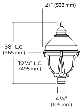
XL10 (shown w/globe) EPA: 1.91 sq.ft. Weight: 40 lbs. (18.1kg)
