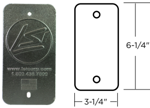
Part #349593CLR Used on all square steel poles and all round steel poles 18'-0" and above except Round Tapered Steel.
