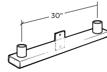
BKS FBO 30 CLR Part # 133163CLR
