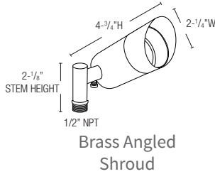
•ANGLED SHROUD
