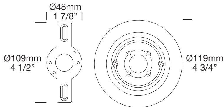
USA Wall Box Adaptor and Wall Plate (Included with USA Wall Mount fixtures)
