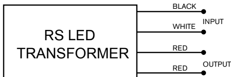
WIRING DIAGRAM
