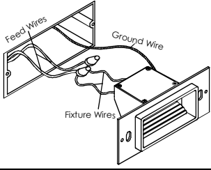
Drawing 2 – Indoor Application
