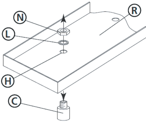
Drawing 2 – Canopy Assembly
