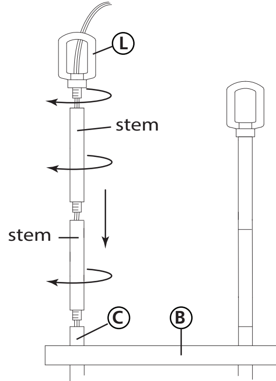
DRAWING 1 - ASSEMBLY
