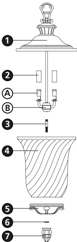
Drawing 1 - Fixture Assembly
