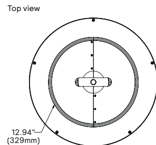
BXS Bird excluding shroud
