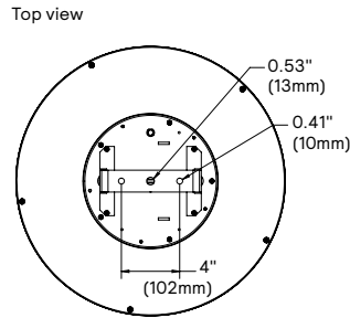
Trunnion mount
