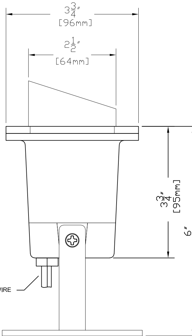
SIDE VIEW WITH DIMENSIONS
