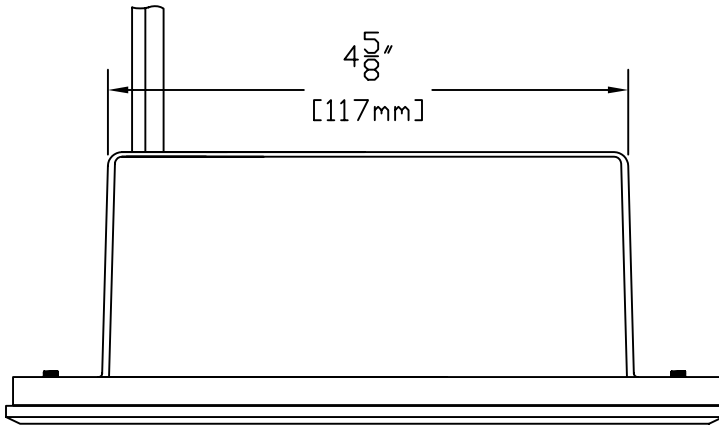
TOP VIEW WITH DIMENSIONS
