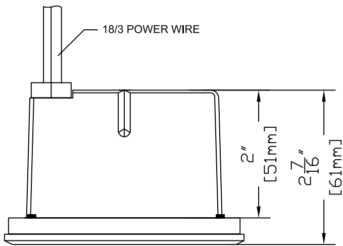
TOP VIEW WITH DIMENSIONS
