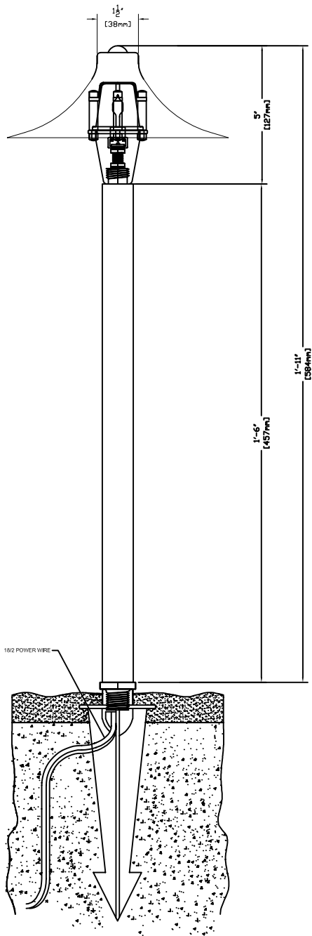
SIDE VIEW WITH DIMENSIONS
