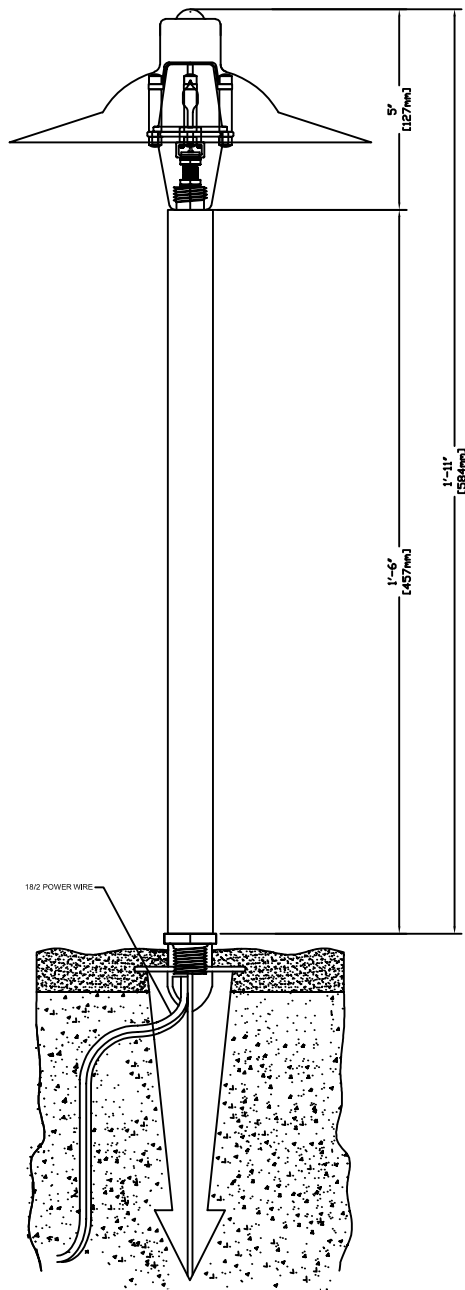
SIDE VIEW WITH DIMENSIONS
