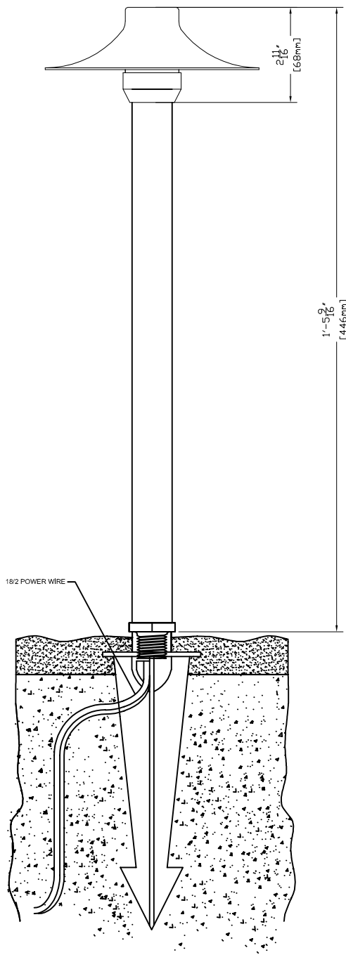
SIDE VIEW WITH DIMENSIONS
