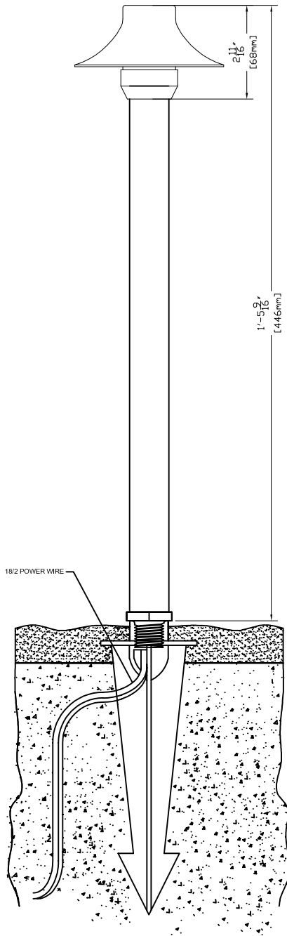
SIDE VIEW WITH DIMENSIONS
