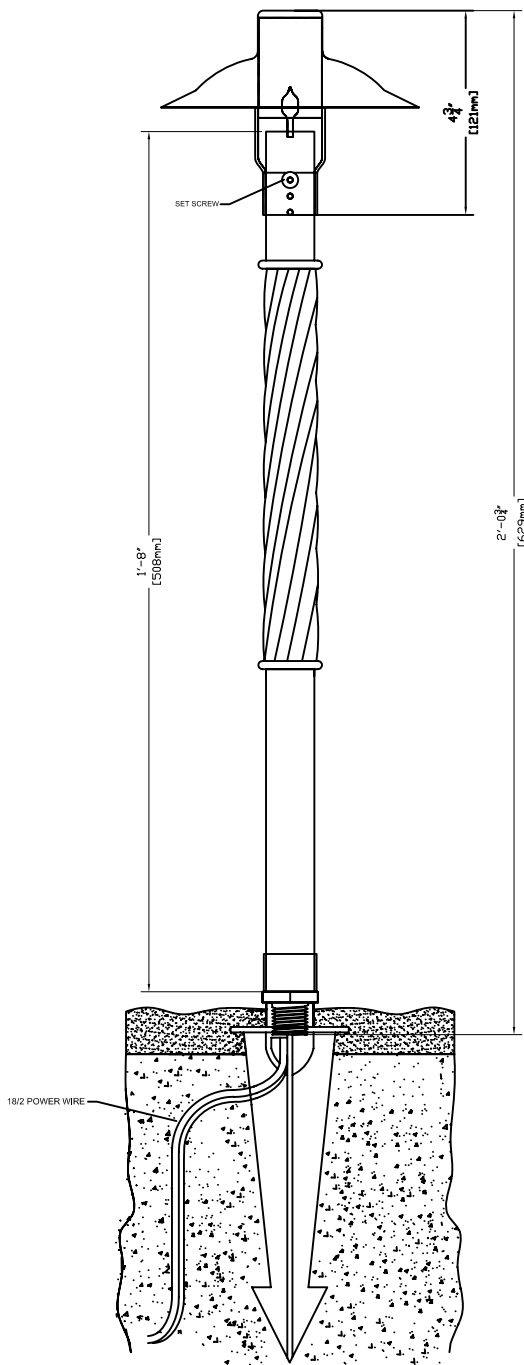
SIDE VIEW WITH DIMENSIONS
