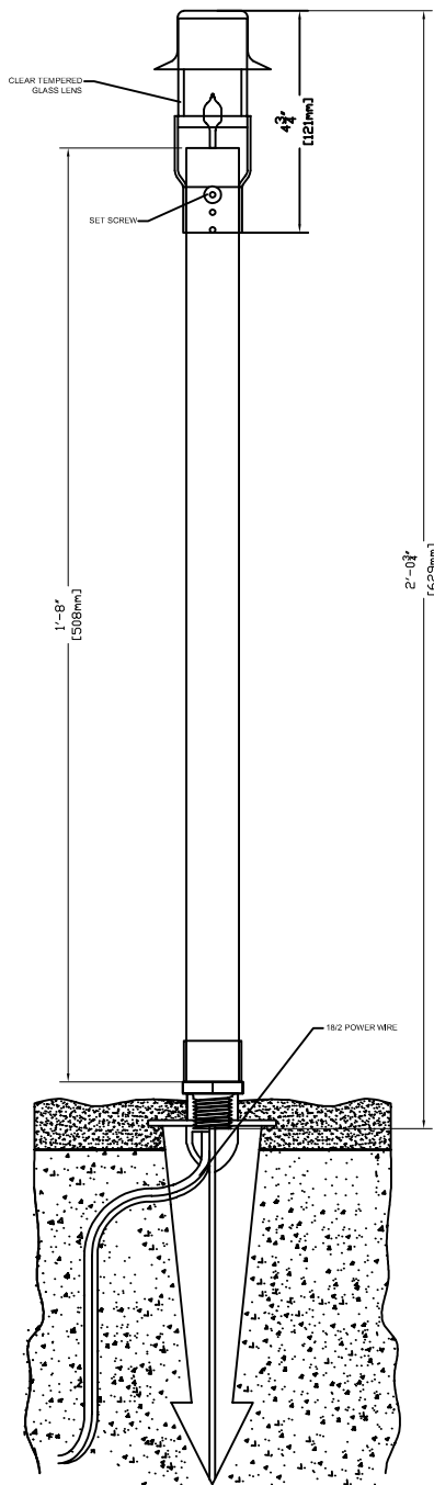
SIDE VIEW WITH DIMENSIONS
