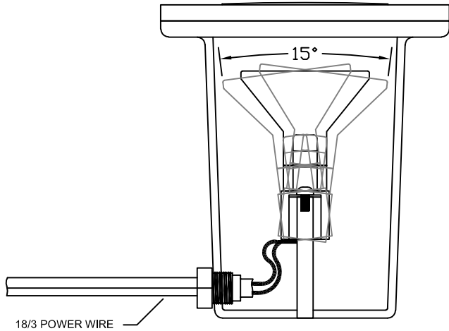
SIDE VIEW WITH ROTATION
