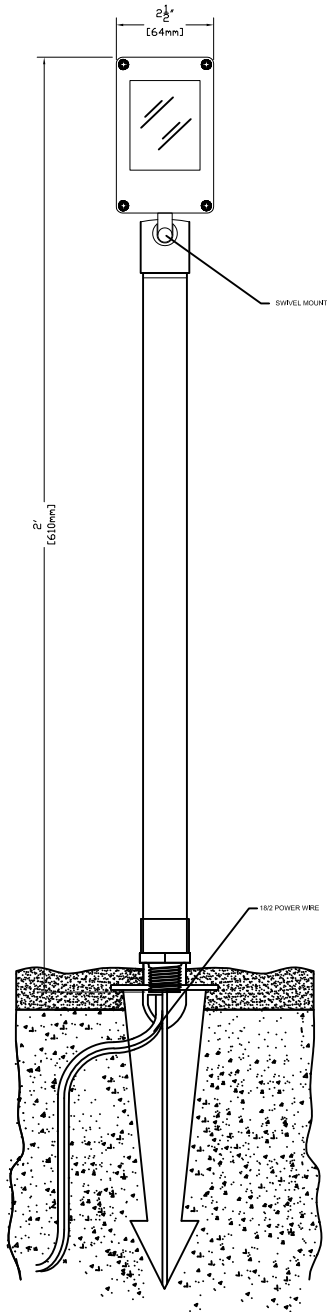
SIDE VIEW WITH DIMENSIONS
